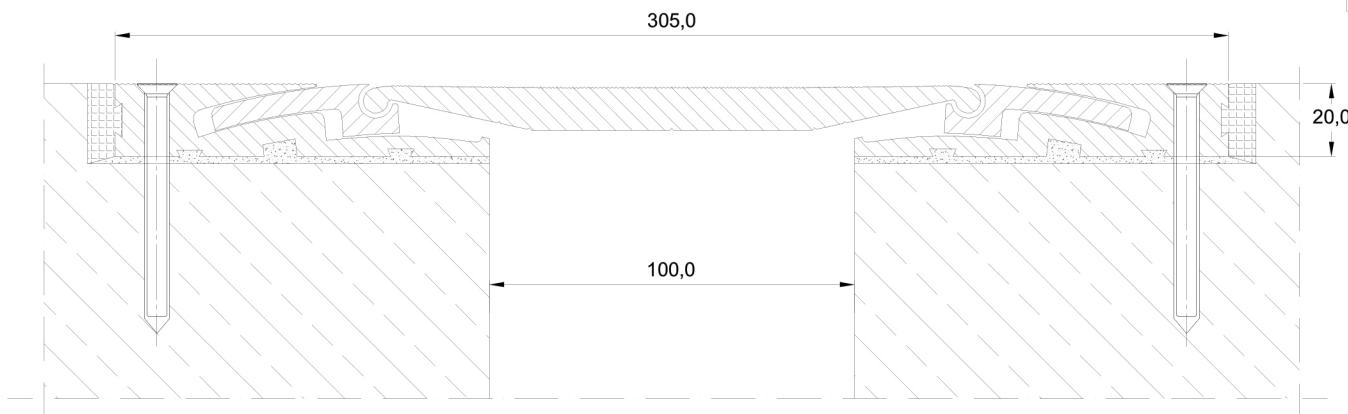
Conecto HDS 100 Section
