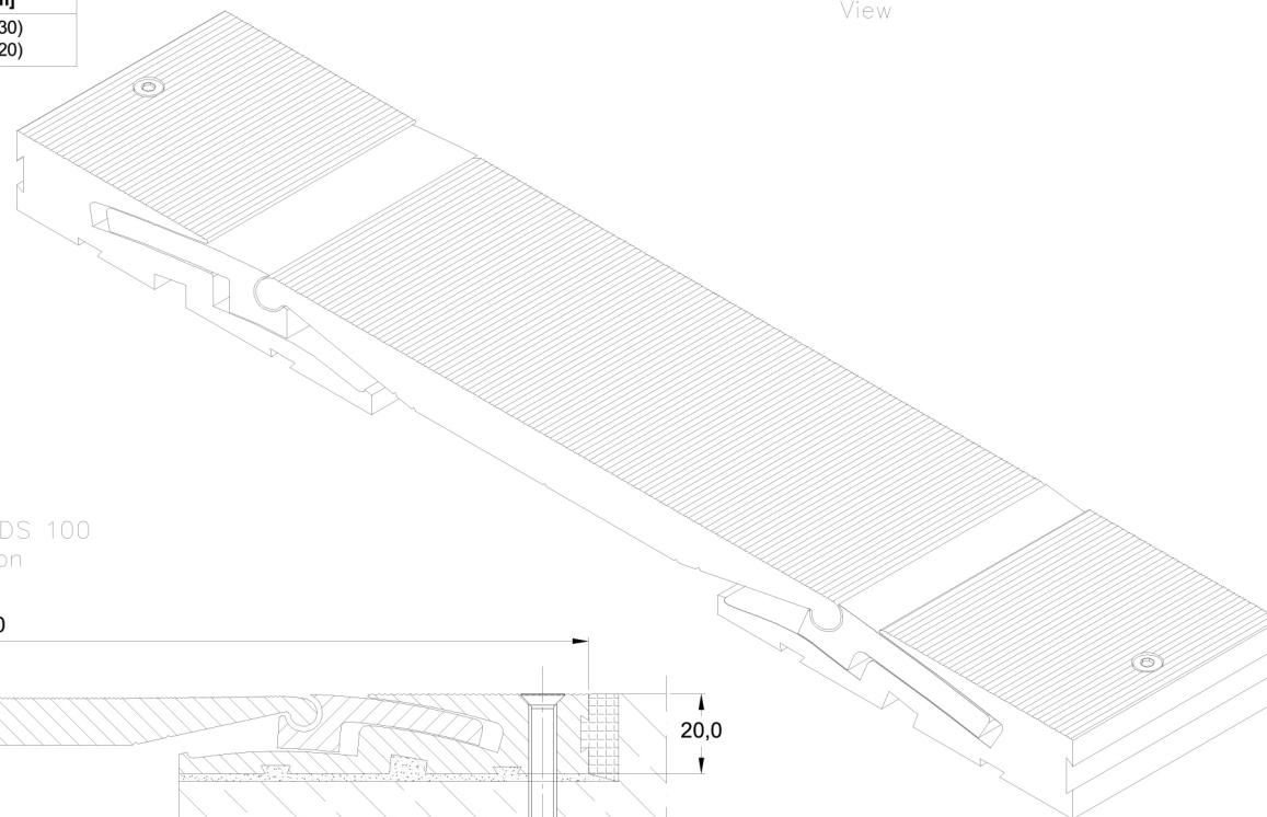
Conecto HDS 100 View
