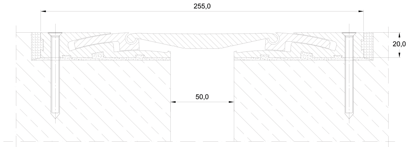
Expansion joint Conecto HDS 50
