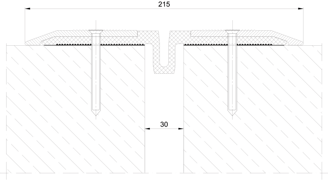
Expansion joint Conecto SL 190.30.N
